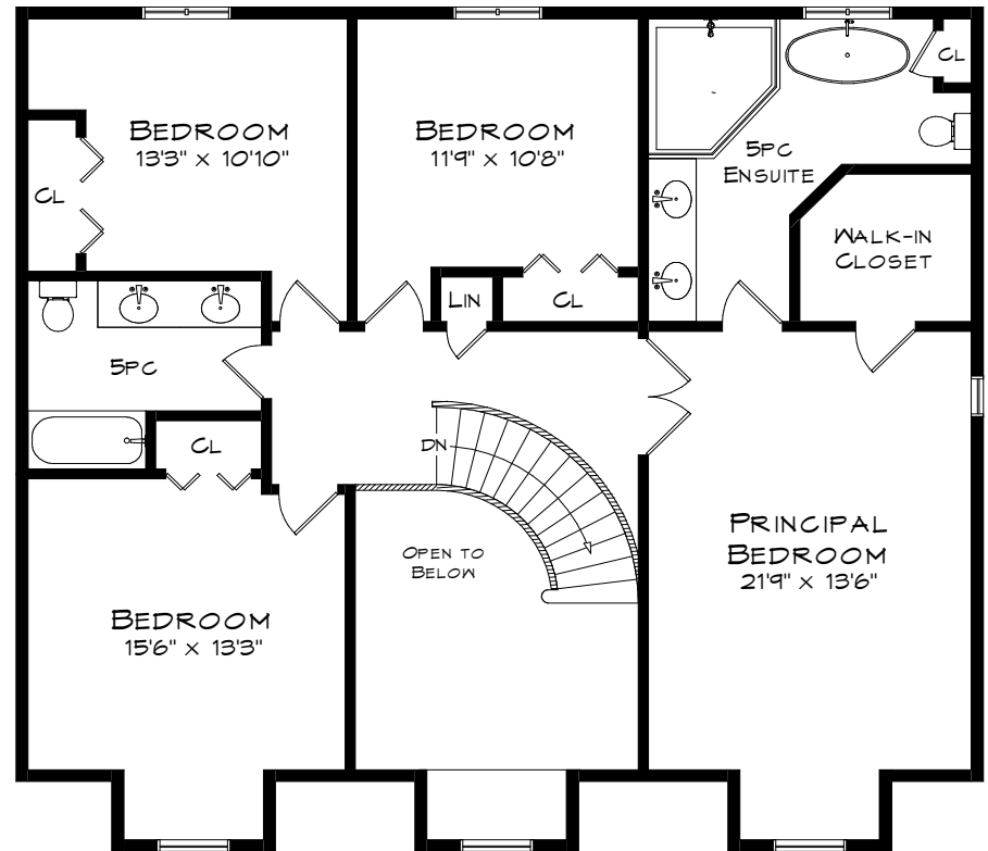
UPPER LEVEL 1,247 SQUARE FEET + 161 SF (OPEN TO BELOW)
